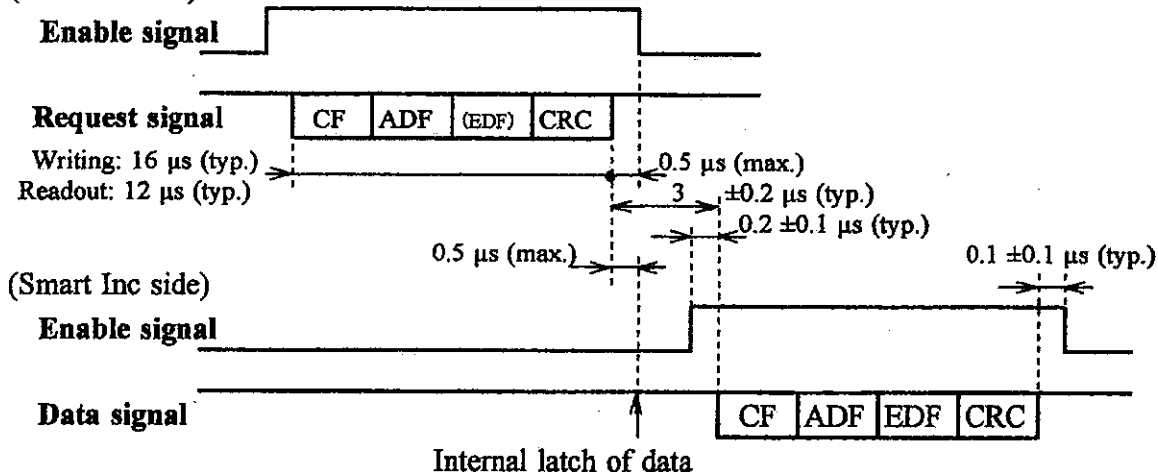
Figure 10. Detection of Frame
