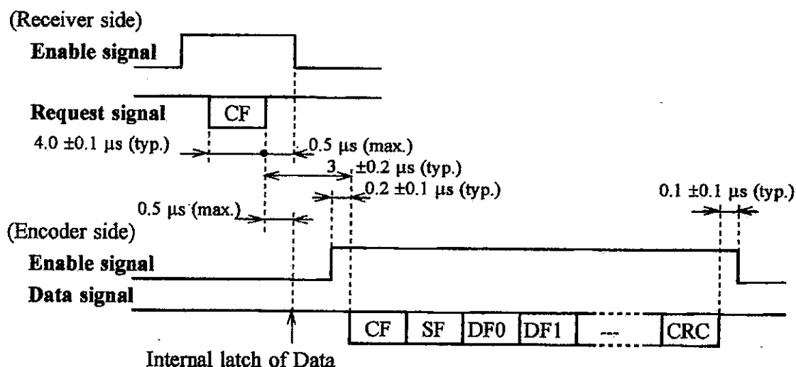
Figure 9. Detection of Frame
