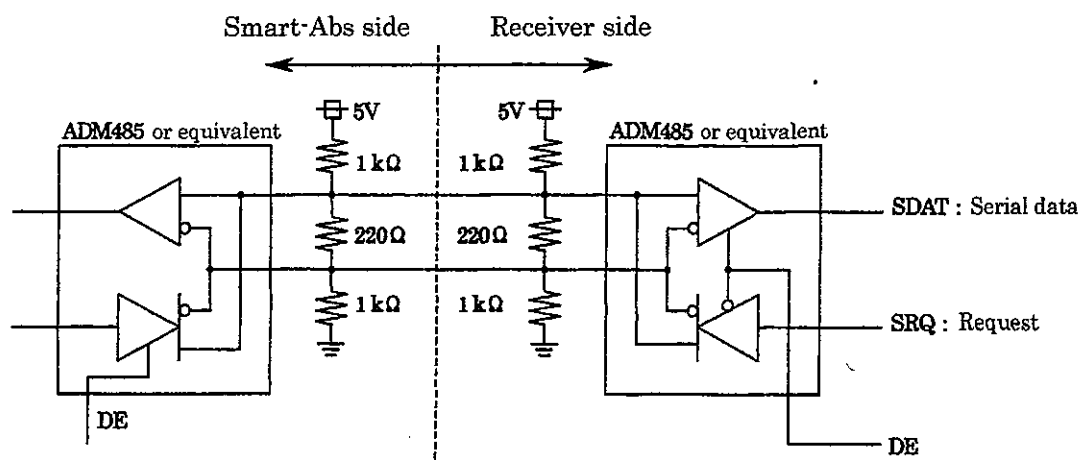
Figure 11. Example of Transmitter and Receiver Circuit
