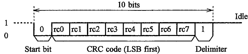
Figure 7. Structure of CRC Field
