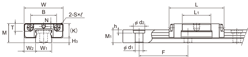
Модели SRS5M, SRS5N
