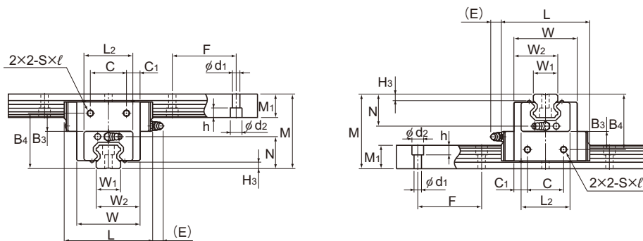
Модели CSR15, 20S до 30S
